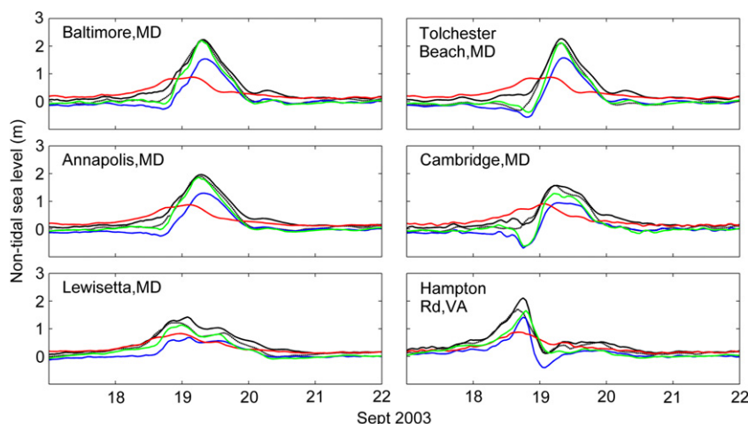
Fig. 11. Time series comparison of the subtidal sea-level elevations from OBS (observed; dashed), and CTRL (control; black solid), with Group E sensitivity simulations: NTID (no incoming coastal storm surge; blue), NWND (no local wind forcing; red) and BIGC (big-domain model run with the control wind fields; green).
